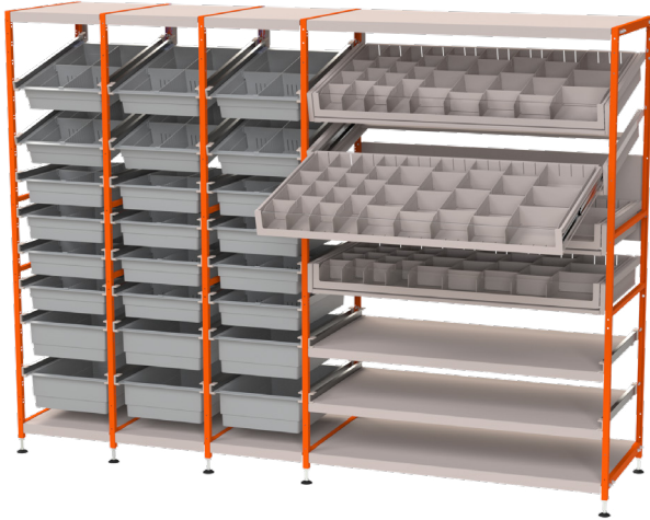
Triple base 600 x 400 + extension 1200 x 600
